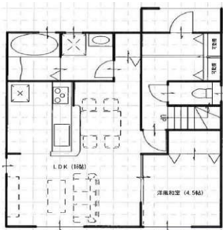
1F 52.99㎡
