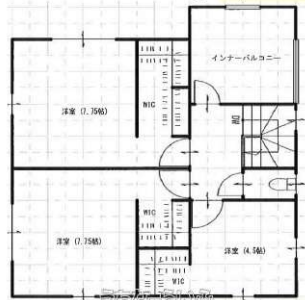
2F 48.03㎡
